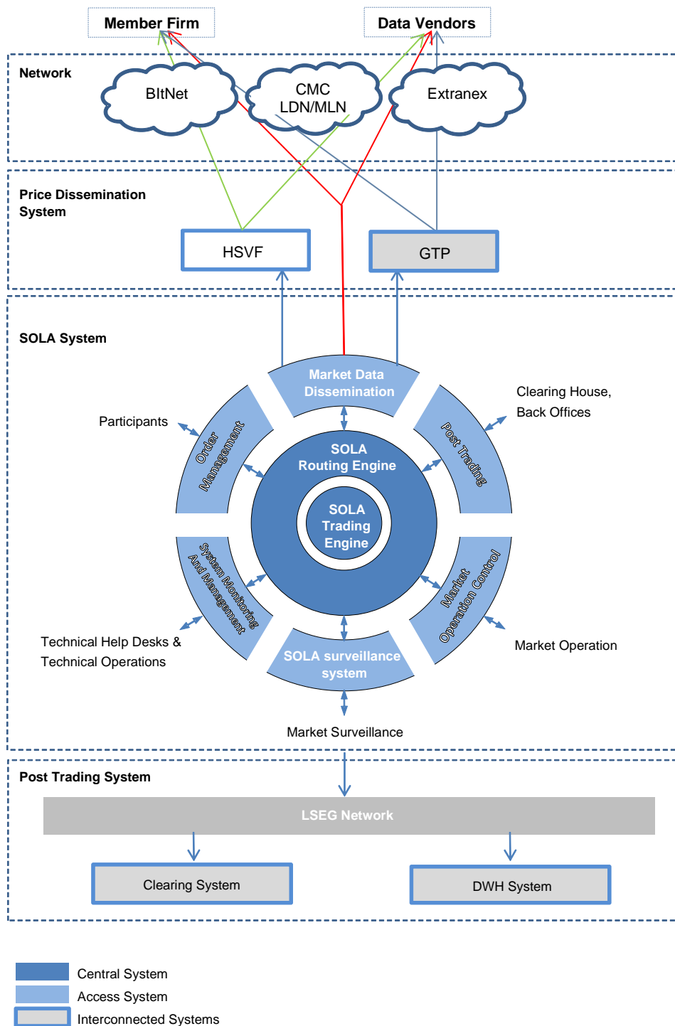
Figure 1: Logical architecture of the IDEM Trading System
